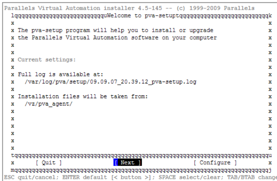
Figure 14: Installing From TUI - Beginning Installation
